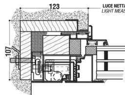
NODO LATERALE E SUPERIORE SIDE AND UPPER NODE CERNIERA A SCOMPARSA / CONCEALED HINGE
